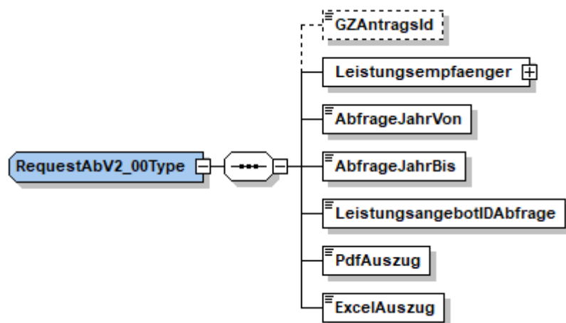
Abbildung 3: RequestAbV2_00Type
